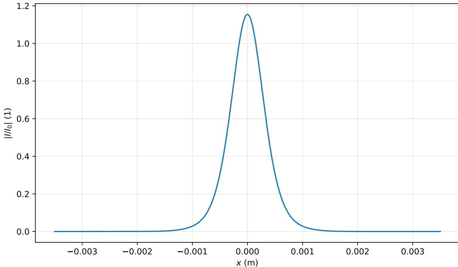
Intensity profile I(x, y = 0, z = 1.751m)/I_0 , P_{in}=0.7P_{cr} , artificial time
